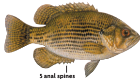
5 anal spines
