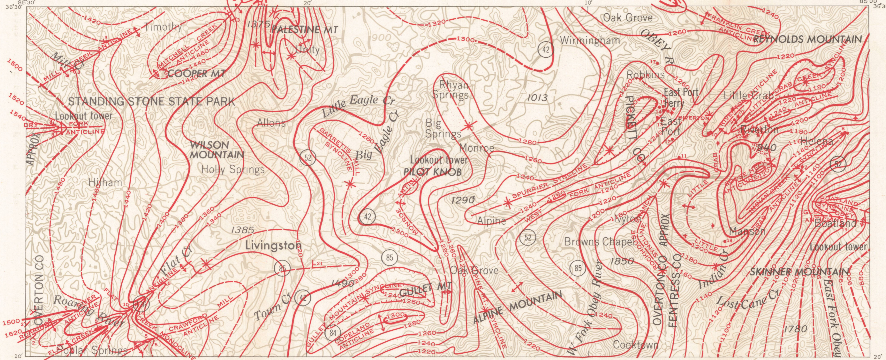
MAP OF THE NORTHERN PART OF OVERTON COUNTY AND PARTS OF ADJACENT COUNTIES IN TENNESSEE, SHOWING GEOLOGIC STRUCTURE
