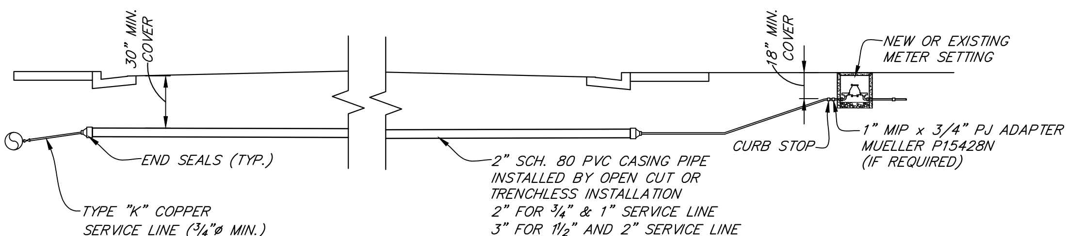
TYPICAL SERVICE LINE CROSSING HIGHWAY
