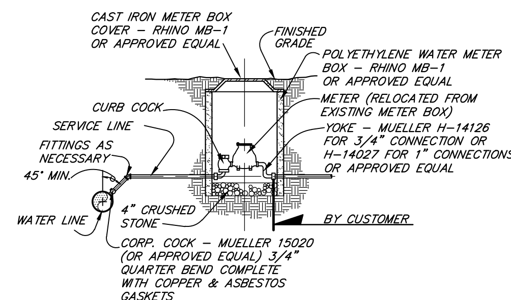
METER SETTING FOR 3/4" OR 1" SERVICES
