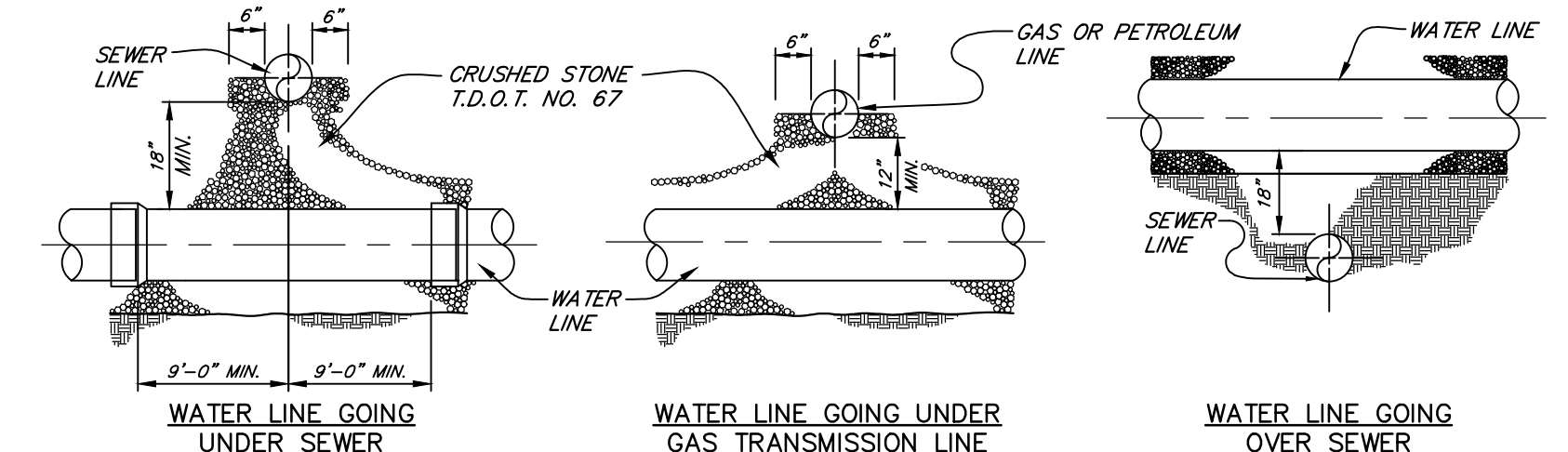
TYPICAL PIPE CROSSING
