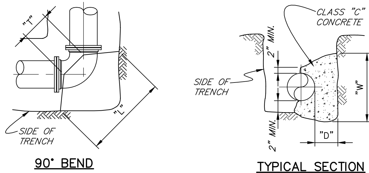
TYPICAL SECTION
