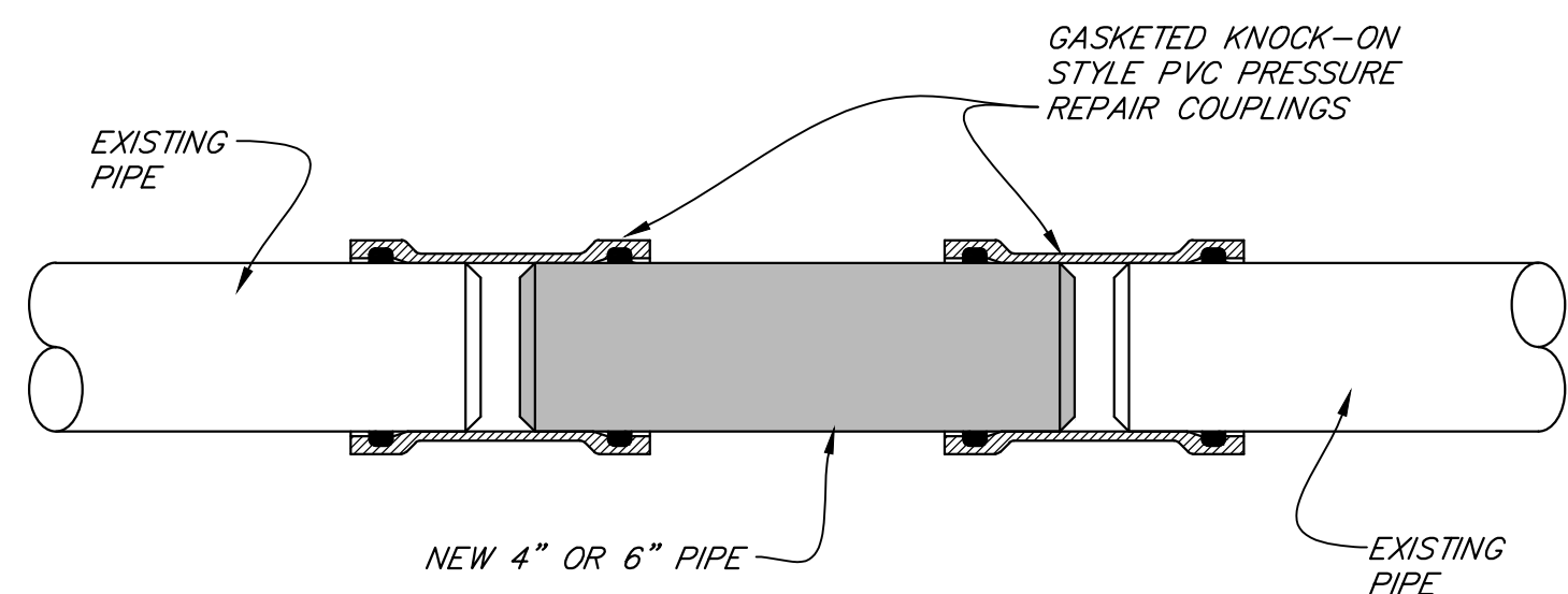
KNOCK-ON STYLE REPAIR COUPLING
