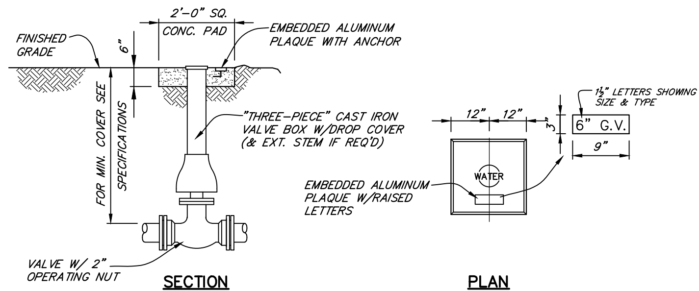
TYPICAL LINE VALVE SETTING
