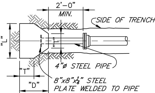
PLUG
