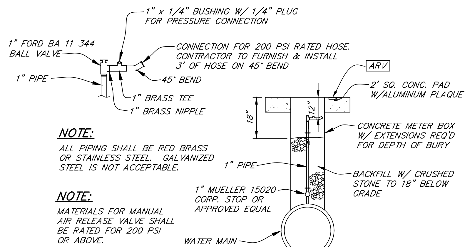
1" MANUAL AIR RELEASE VALVE ASSEMBLY
