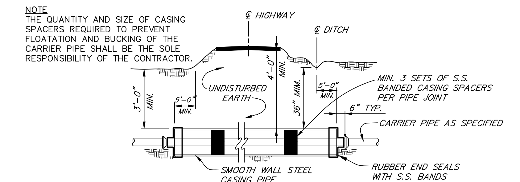
BORED HIGHWAY CROSSING DETAIL
