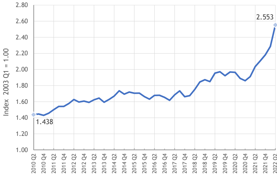
Figure 17. National Highway Construction Cost Index (NHCCI) 2 nd Quarter 2010 through 2 nd Quarter 2022
