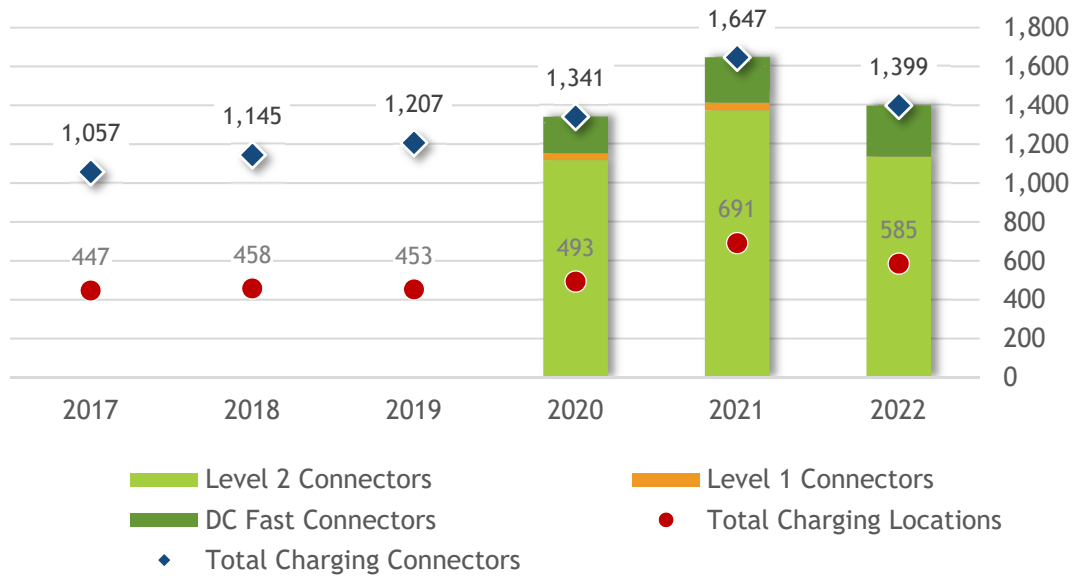
Figure 10. Electric Vehicle Charging Stations in Tennessee 2017 through 2022*
