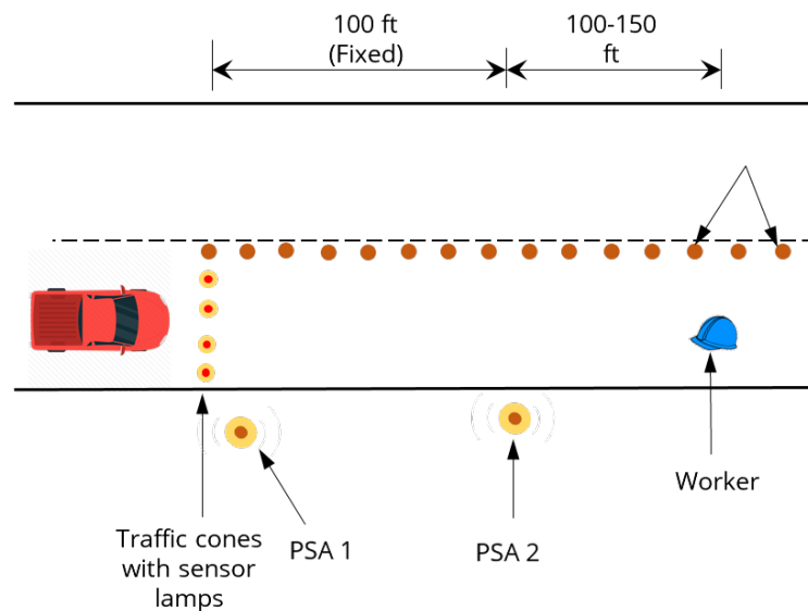
Figure 4-11. Experimental setup for testing alarm activation and worker response
