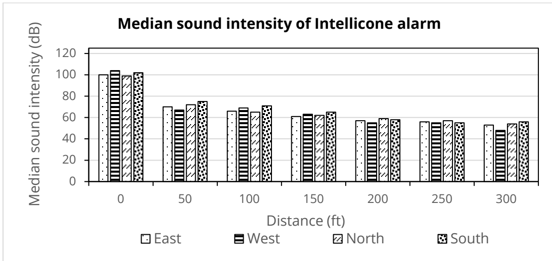
(a) Variation of intensity with distance and direction: Intellicone
