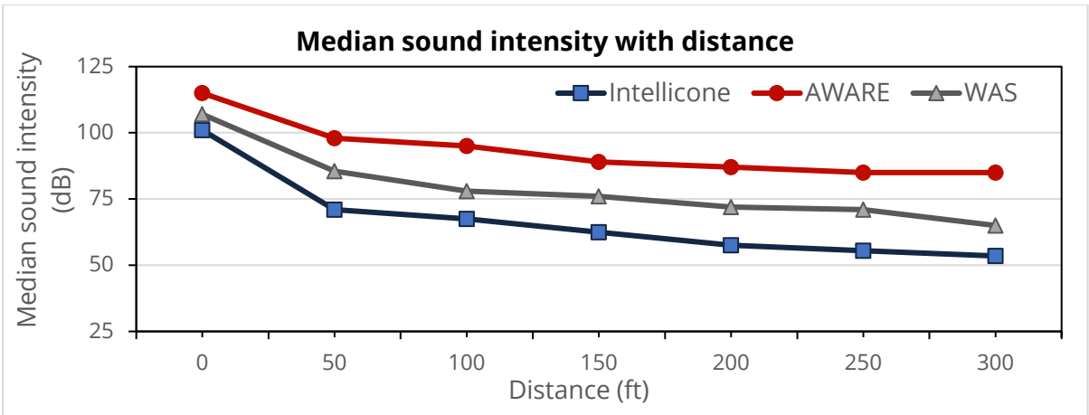
Figure 4-7. Variation in the sound intensity of alerts with distance
