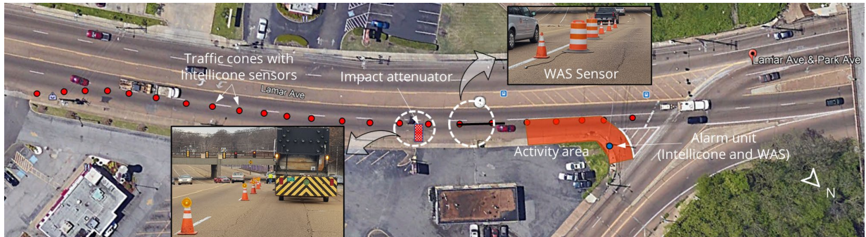
Figure 4-29. Project 3: Arrangement of Intellicone and WAS components.
