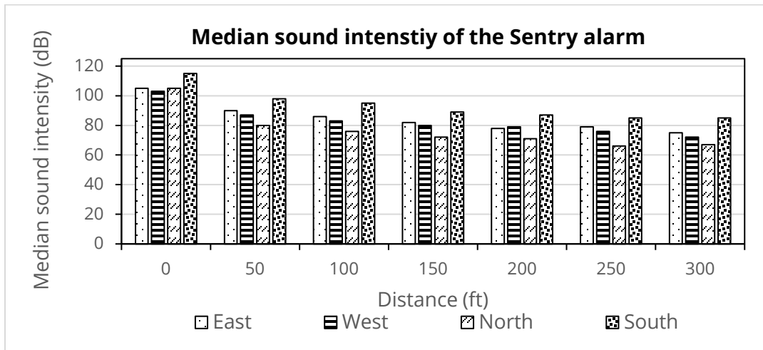
(b) Variation of intensity with distance and direction: AWARE Sentry
