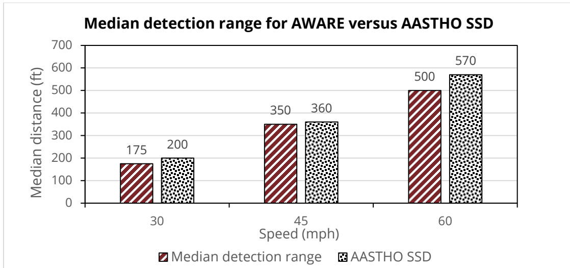
Figure 4-17. Detection range for the Sentry compared with AASTHO SSD
