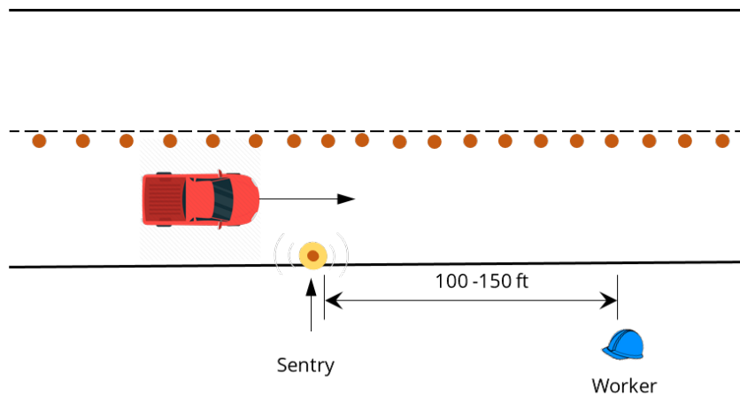
Figure 4-15. Experimental arrangement for testing AWARE Sentry: Scenario 2
