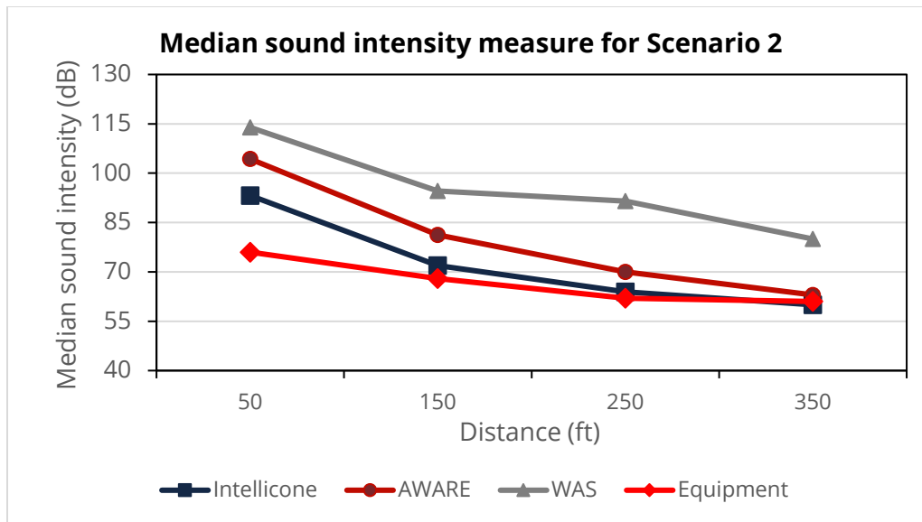
Figure 4-24. Results from experimental evaluating sound intensity in presence of equipment: Scenario 2
