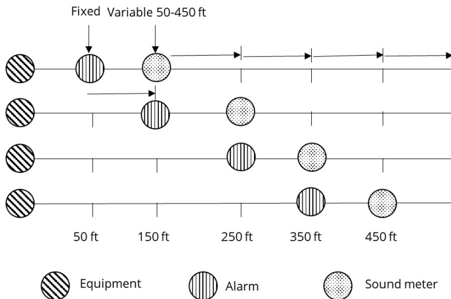
Figure 4-23. Experimental arrangement for evaluating sound intensity in presence of equipment: Scenario 2
