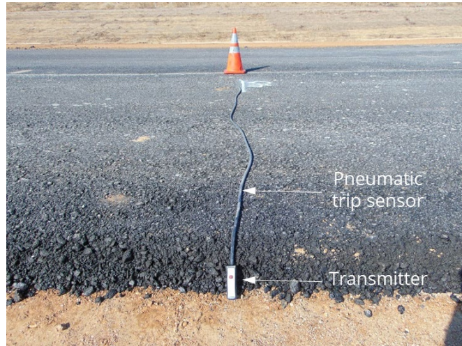
(a) Pneumatic sensor hose
