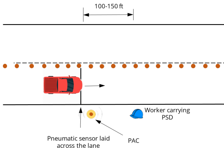
Figure 4-18. Experimental arrangement for testing WAS
