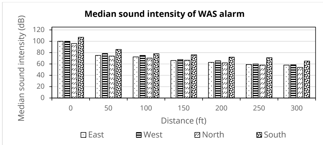
(c) Variation of intensity with distance and direction: WAS
