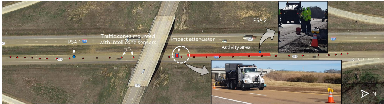
Figure 4-27. Project 2: Arrangement of Intellicone components
