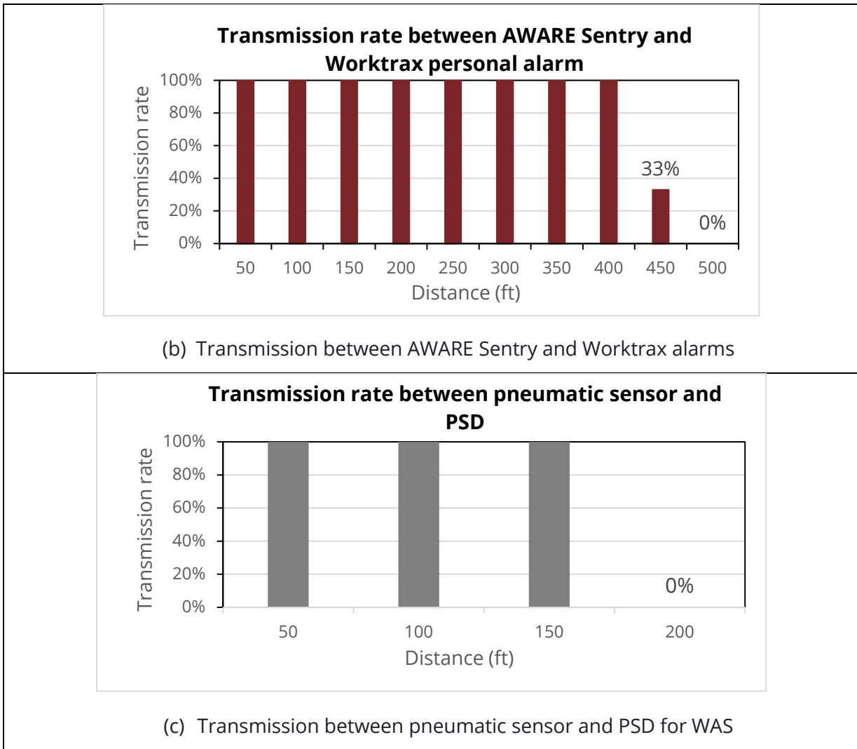
Figure 4-10. Transmission range of different technology components
