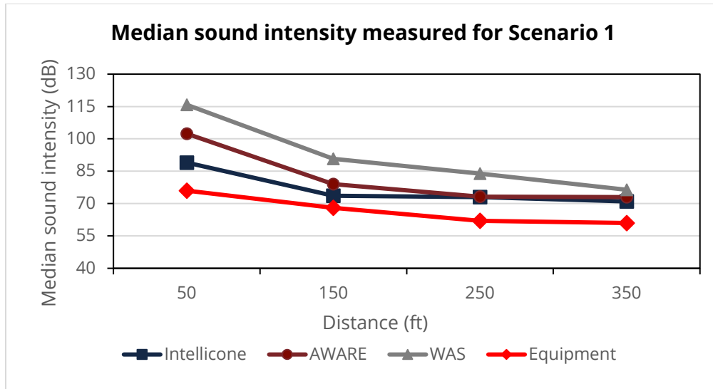
Figure 4-22. Results from experimental evaluating sound intensity in presence of equipment: Scenario 1
