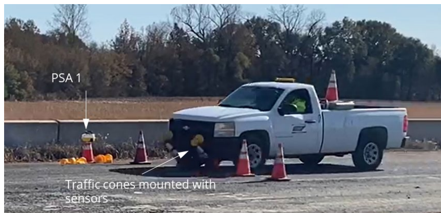
Figure 4-12. Crash testing of Intellicone sensors
