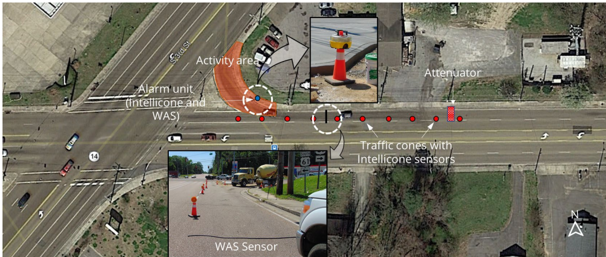
Figure 4-33. Project 5: Arrangement of Intellicone and WAS components
