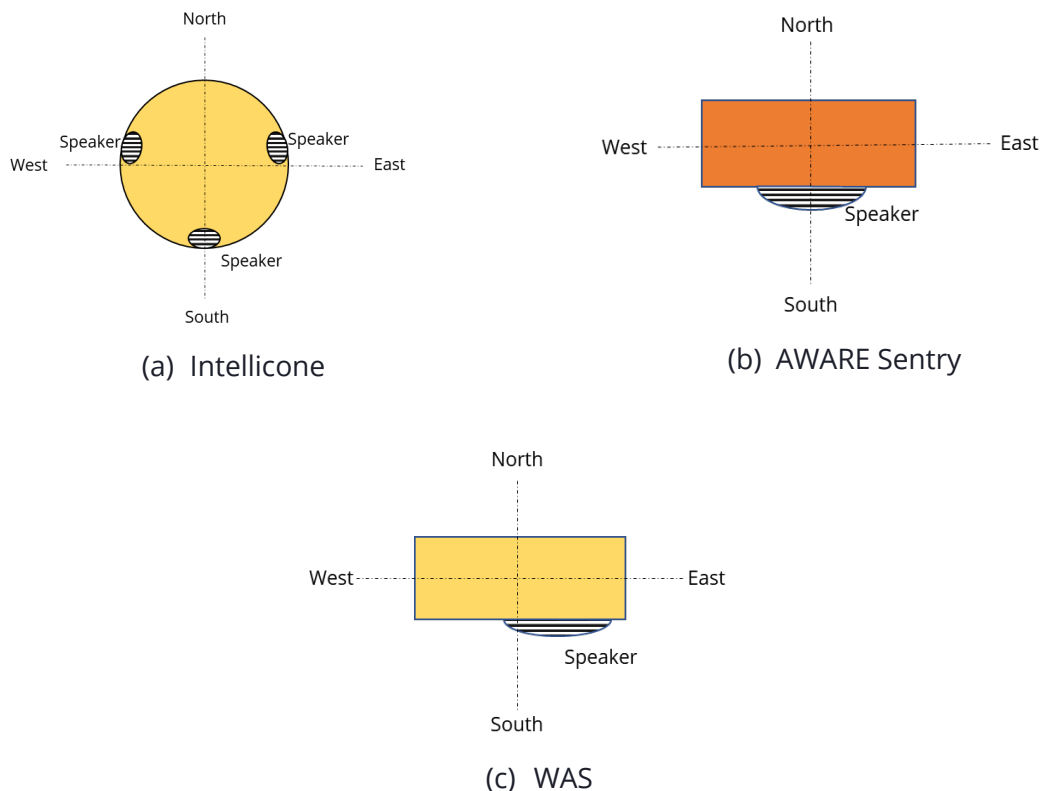
Figure 4-6. Relational directions used in measuring sound intensities of the technologies shown in top view. Placement of alarm speakers within the alarm units is also shown.
