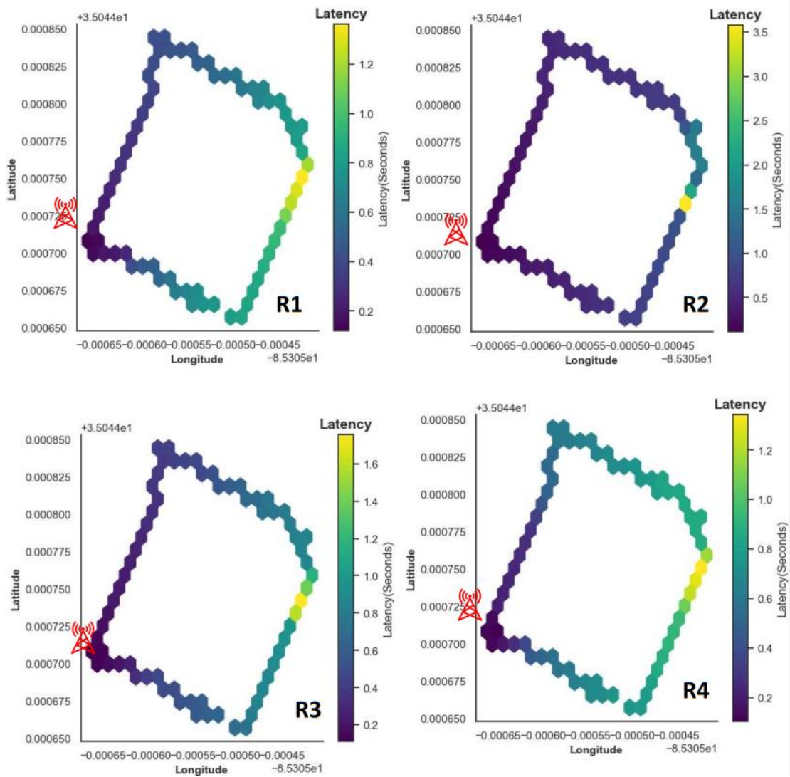
FIGURE 4.8: Hexagonal binnings for latency of LTE communication system at Houston intersection
