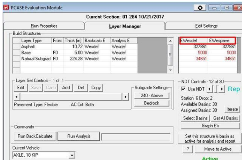
Figure 30: EWesdef and EWespace
