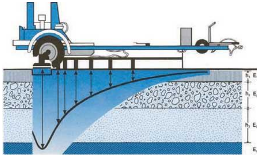
Figure 10: FWD test.
