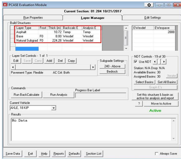
Figure 24: Pavement layers.
