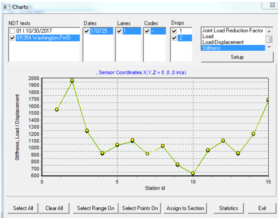
Figure 15: Stiffness Chart
