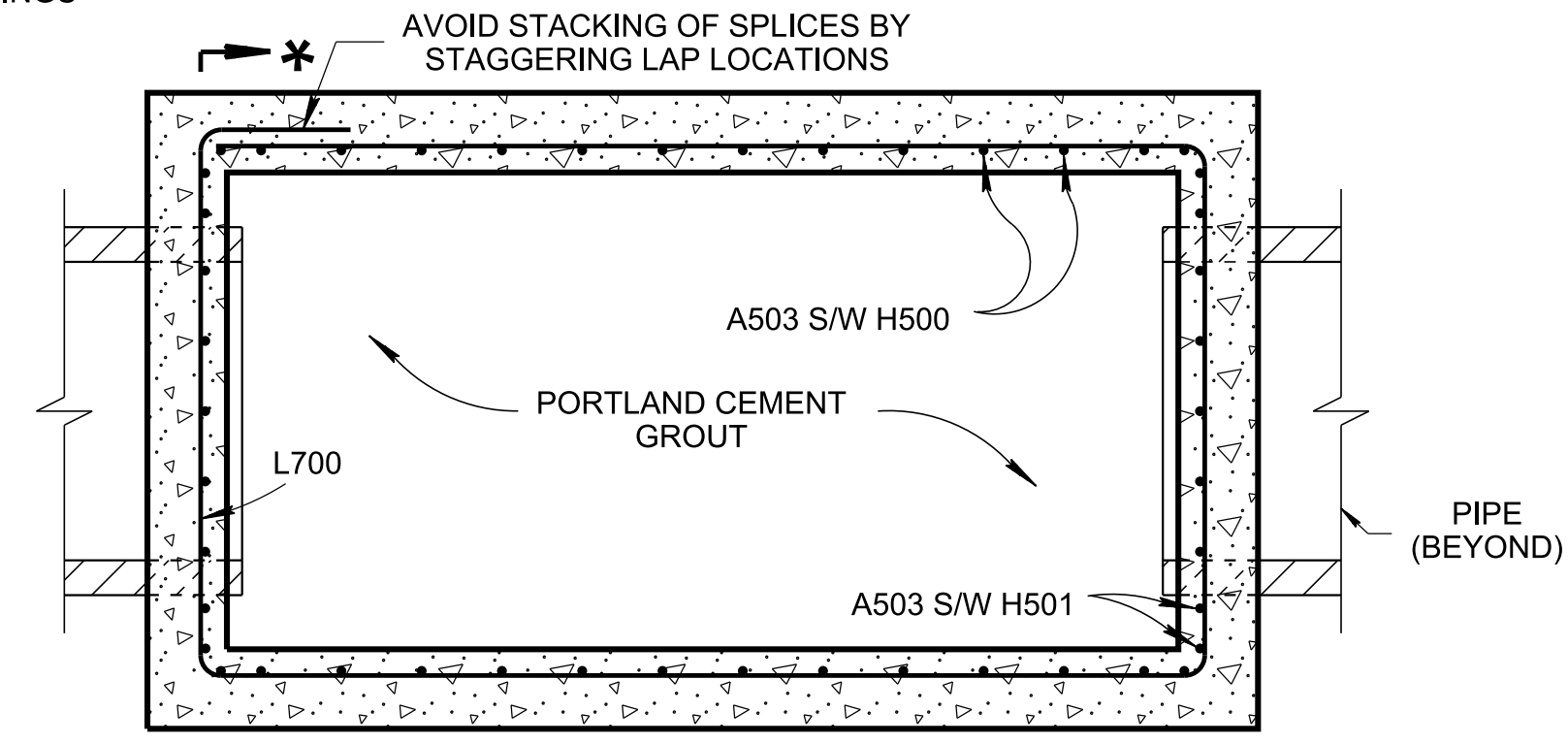
SECTION E-E
