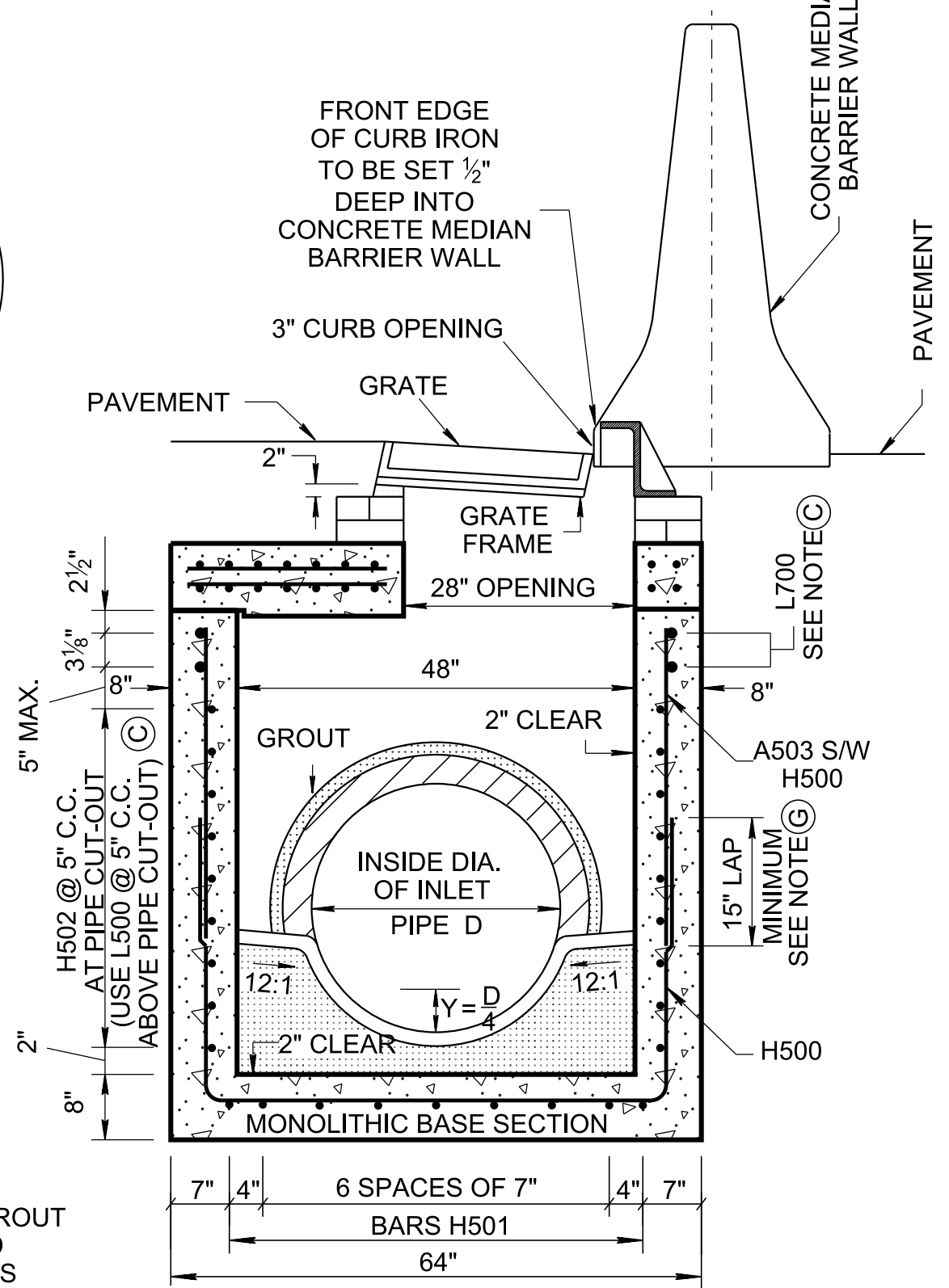
SECTION B-B
