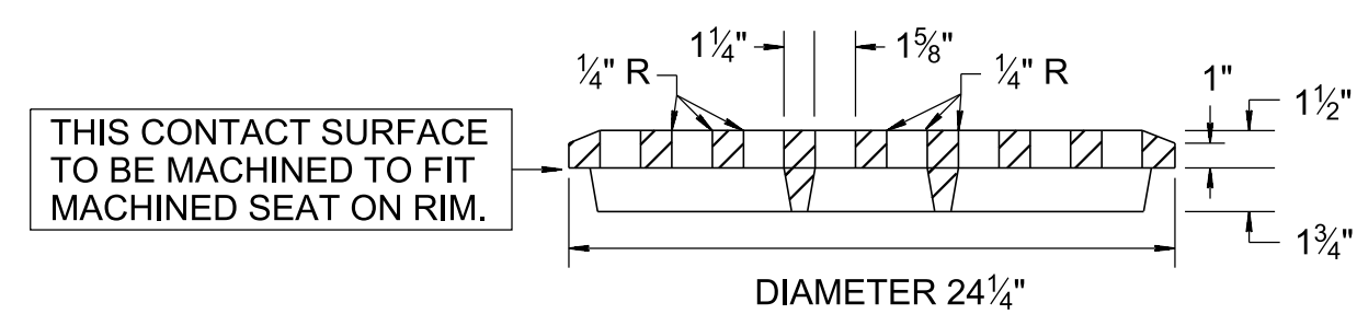
SECTIONAL VIEW
