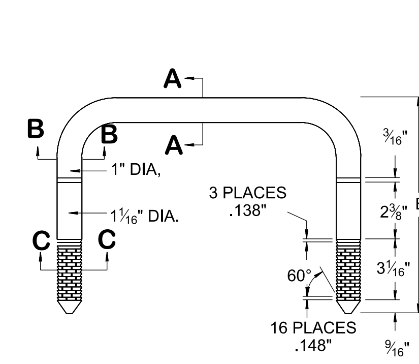
PLAN VIEW
