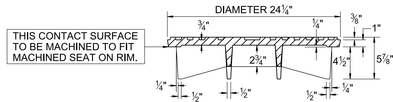
SECTIONAL VIEW FOR TYPE B AND C
