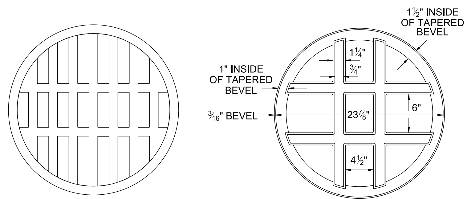
TOP VIEW
