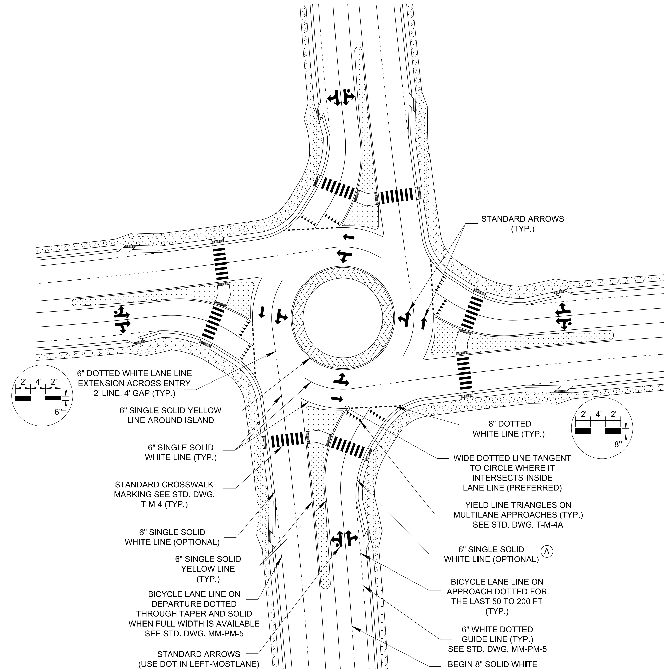
TYPICAL PAVEMENT MARKINGS FOR MULTI LANE ROUNDABOUT
