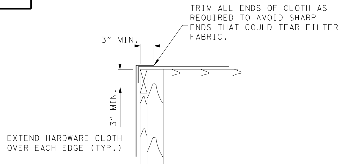
HARDWARE CLOTH OVERLAP DETAIL N.T.S.
