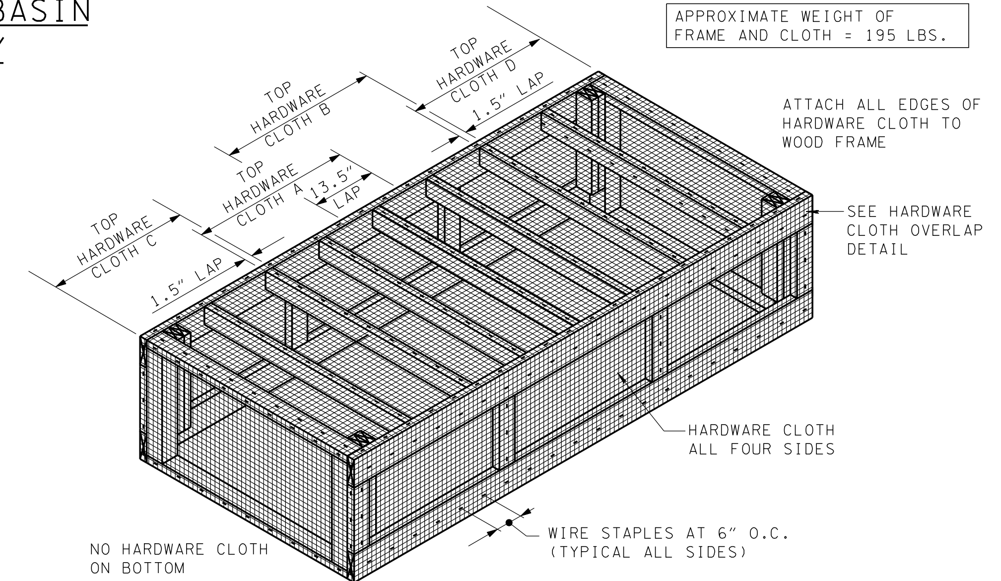
ISOMETRIC VIEW FRAME WITH HARDWARE CLOTH N.T.S.
