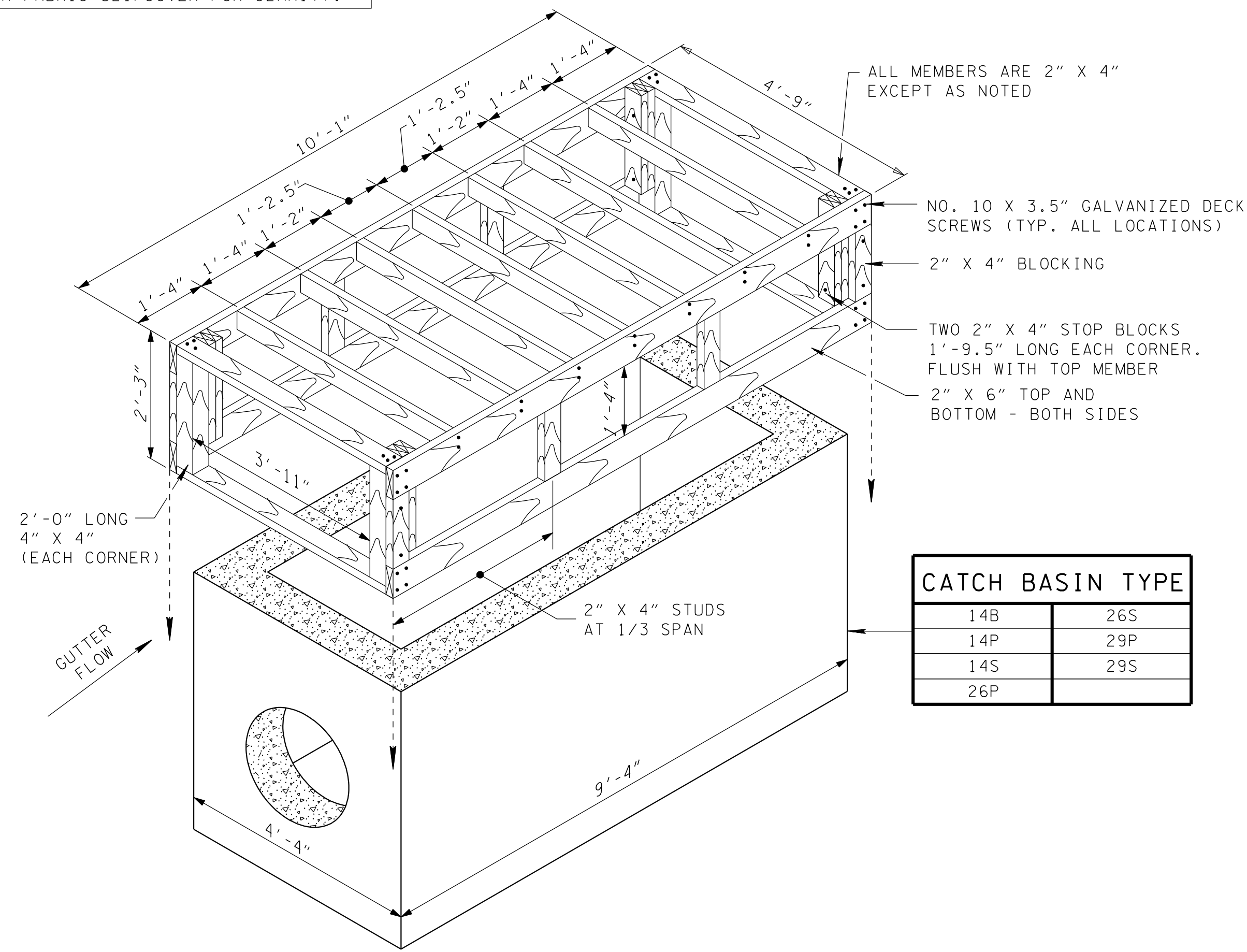
ISOMETRIC VIEW CATCH BASIN FILTER ASSEMBLY N.T.S.
