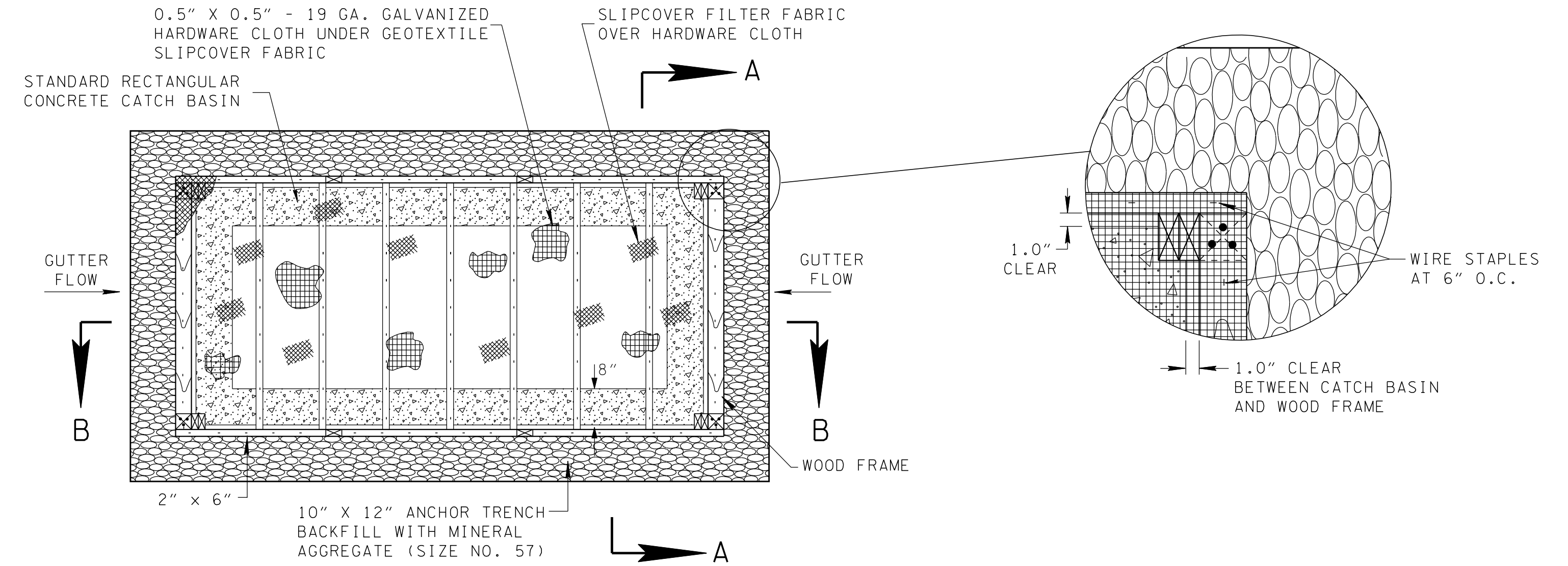
PLAN VIEW - CATCH BASIN FILTER ASSEMBLY N.T.S.
