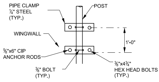
PIPE CLAMP CONNECTION DETAIL
